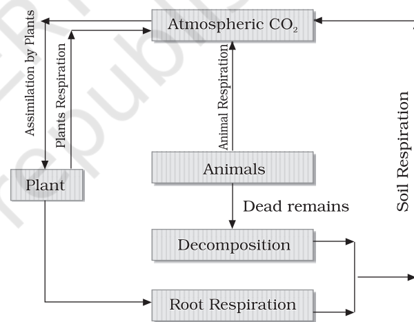
Figure 15.2 : Carbon Cycle
